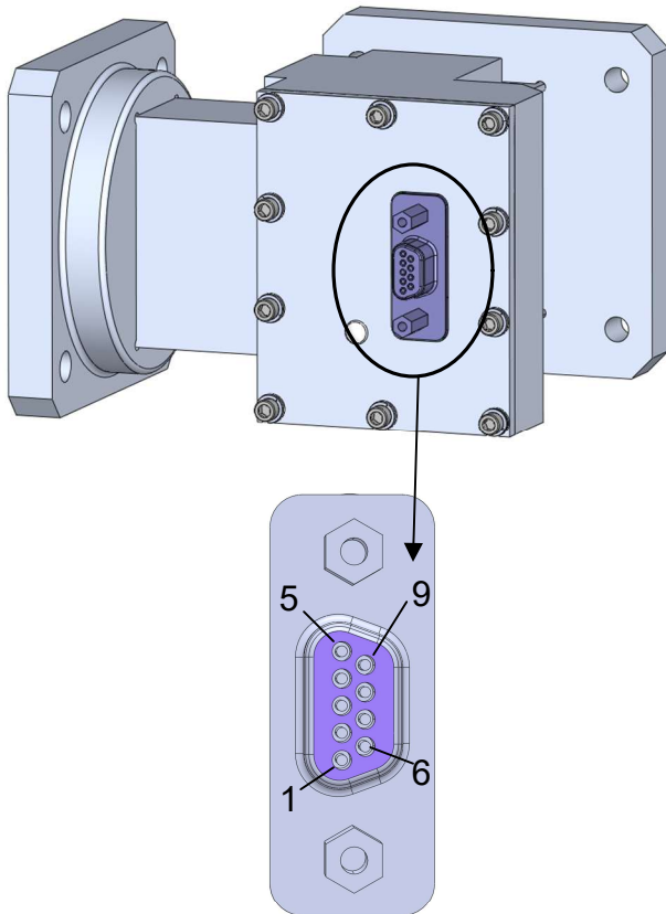
micro D-sub connector
