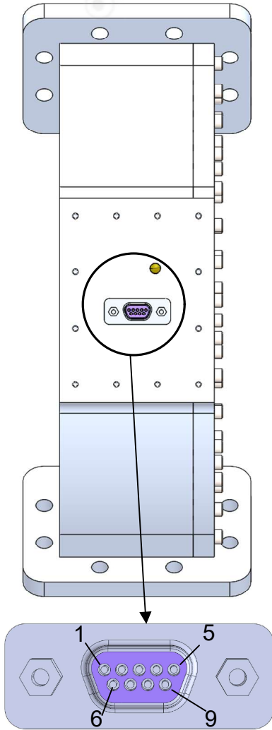
micro D-sub connector
