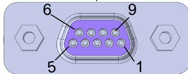
micro D-sub connector
