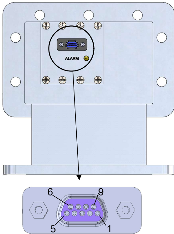
micro D-sub connector
