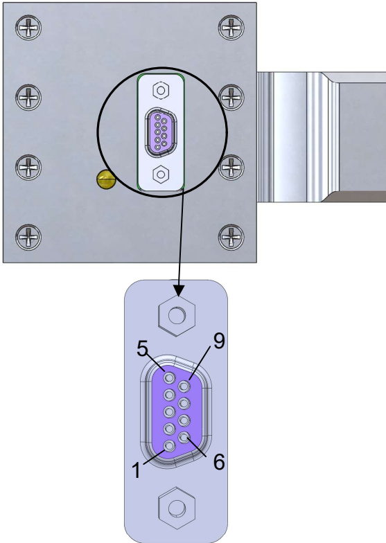
micro D-sub connector
