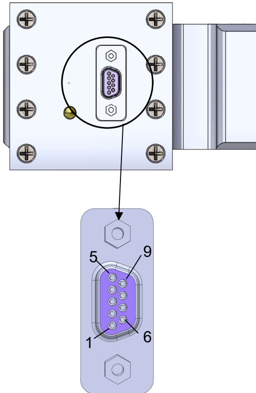
micro D-sub connector
