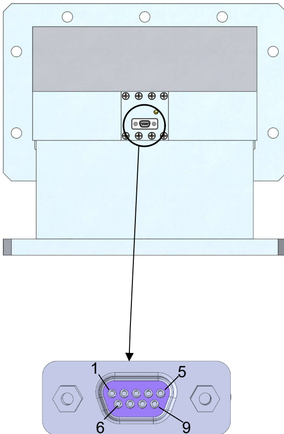
micro D-sub connector
